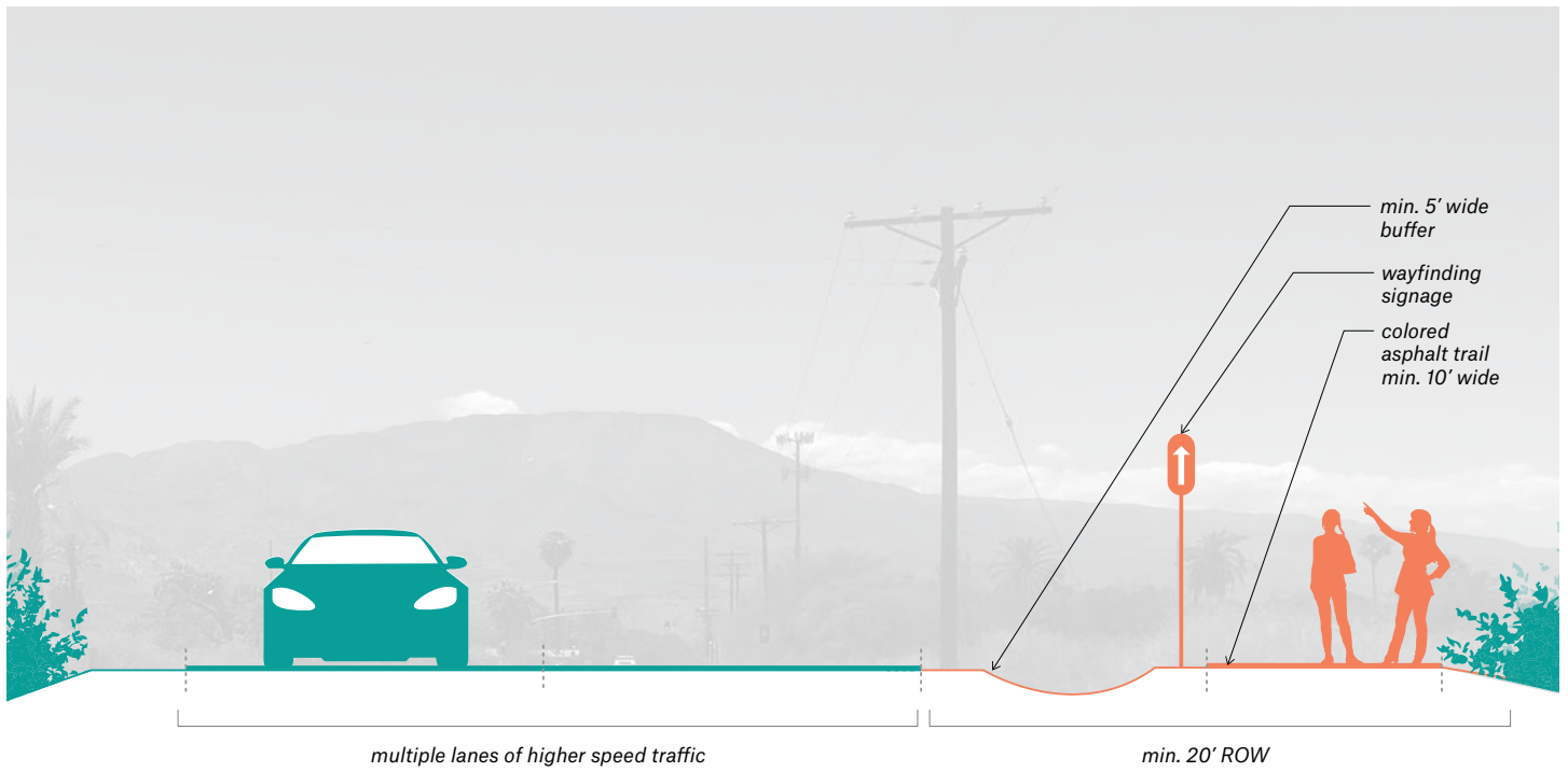
Figure 20. Typical Cross-Section: 10-foot Wide Class I Multimodal Path
