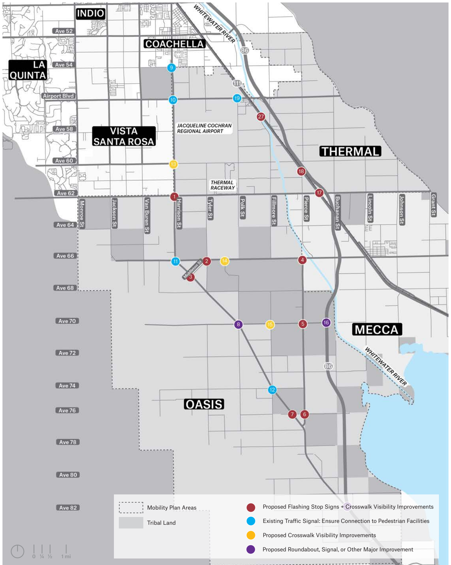
Figure 24. Proposed Intersection and Pedestrian Crossing Improvements
