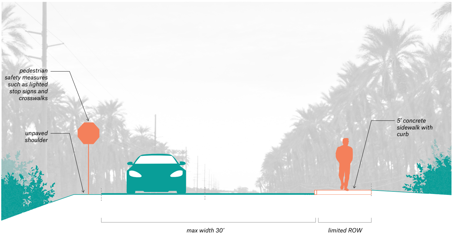
Figure 22. Typical Cross-Section: 5-foot Wide Concrete Sidewalk with Curb
